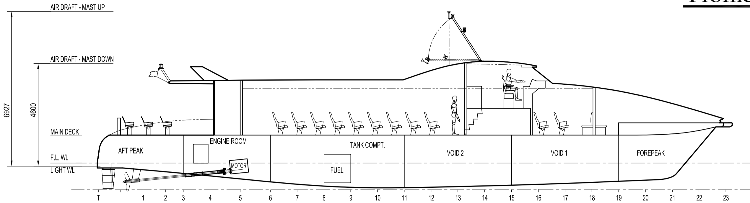
Centreline Profile
