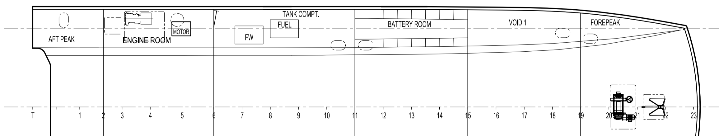
Below Decks
