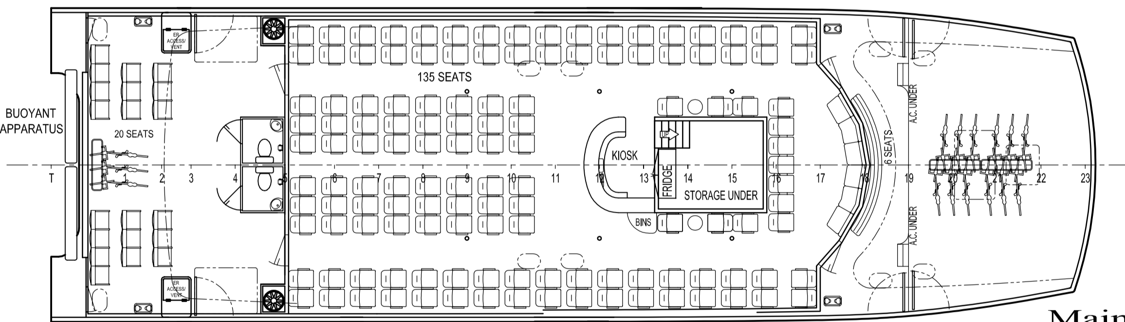
Main Deck
