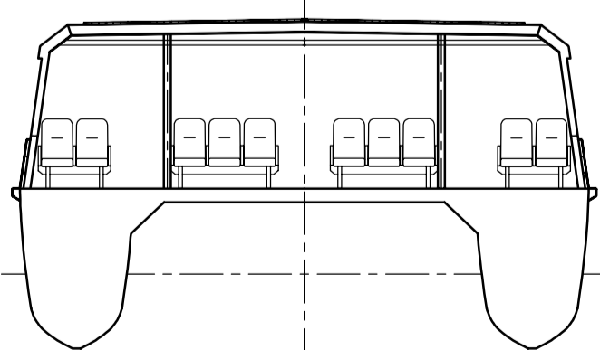
Typical Section
